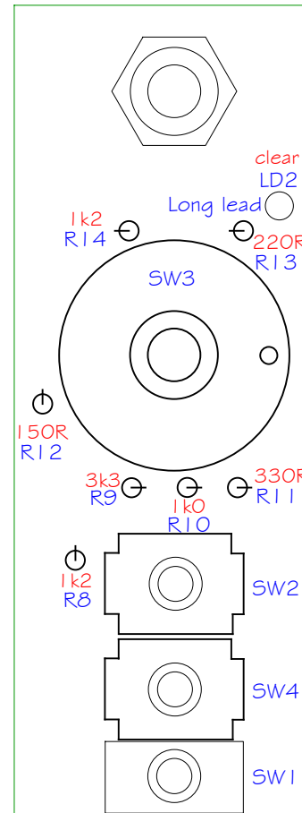
TOP VIEW
