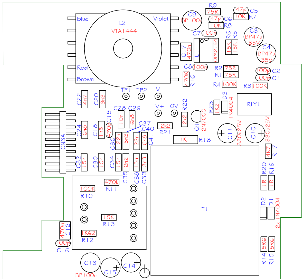
Main PCB
