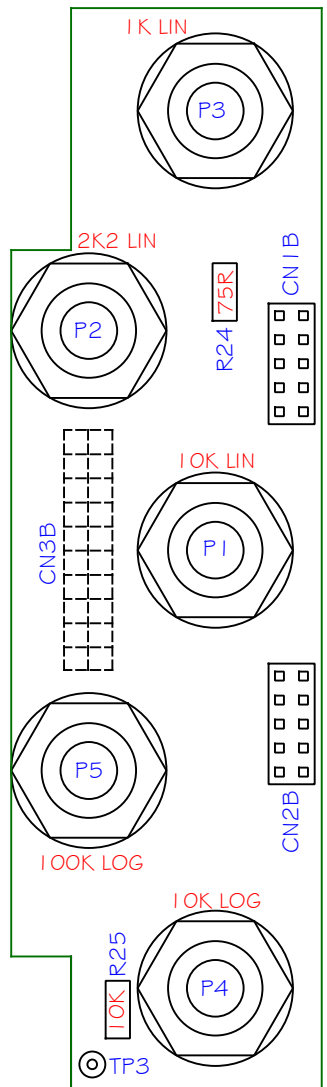
Pots PCB
