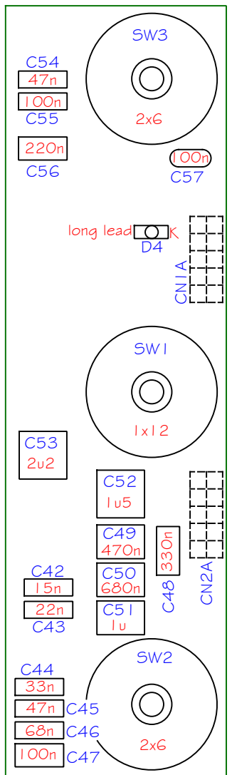
Switches PCB
