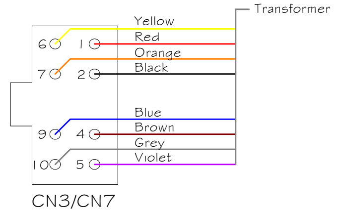
Transformer wiring
