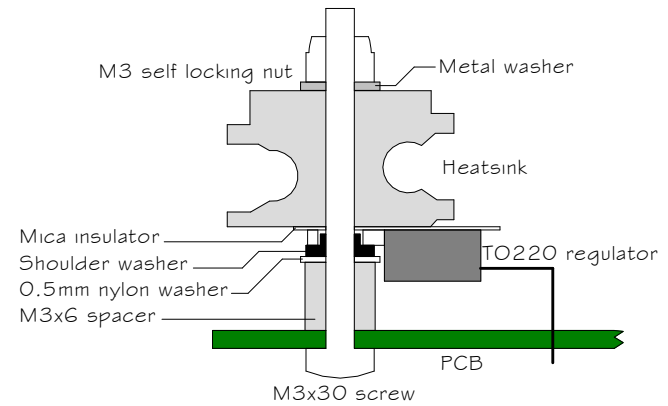
Heatsink Assembly
