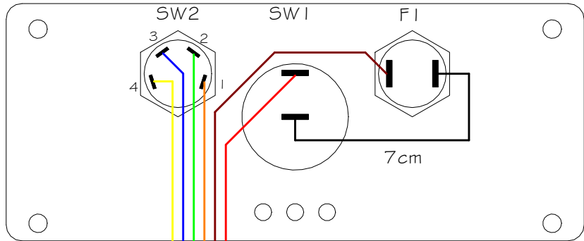
Front pannel wiring
